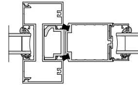
GT55 NI Jamb Locking Stile
