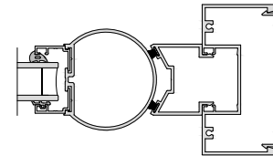
GT55 NI Jamb Anti Finger
